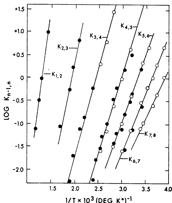
Figure 3. van't Hoff-type plots of equilibrium constants: \circ , \alpha -particle mass spectrometer; \bullet , proton mass spectrometer.
