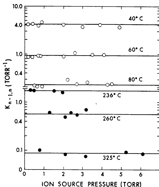
Figure 2. Plot of some representative equilibrium constants K_{n-1,n} for the reaction \text{H}^+(\text{H}_2\text{O})_{n-1,n} + \text{H}_2\text{O} \rightleftharpoons \text{H}^+(\text{H}_2\text{O})_n with water pressure: ○, K_{4,5} obtained with \alpha -particle mass spectrometer; ●, K_{2,3} obtained with proton mass spectrometer.
