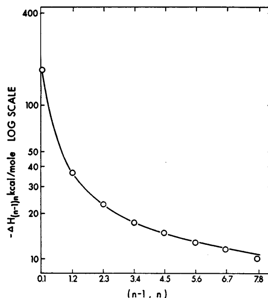
Figure 7. Logarithmic plot of \Delta H_{n-1, n} vs. n-1, n which allows a larger spread of values to be accommodated. Continuous extrapolation of data to \Delta H_{0,1} which is the negative proton affinity of water suggests that, at least for small n , clusters are of the type \text{H}^+(\text{H}_2\text{O})_n where all water molecules are equivalent.
