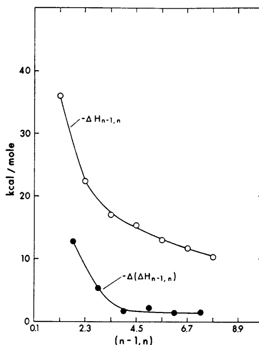
Figure 4. Plot of \Delta H_{n-1,n} and \Delta(\Delta H_{n-1,n}) vs. n-1,n . The enthalpies of the reactions decrease quite regularly. A possible break is indicated between \Delta H_{3,4} and \Delta H_{4,5} . As explained in text, this might be due either to a transition into a new "shell" or crowding of the old "shell."
