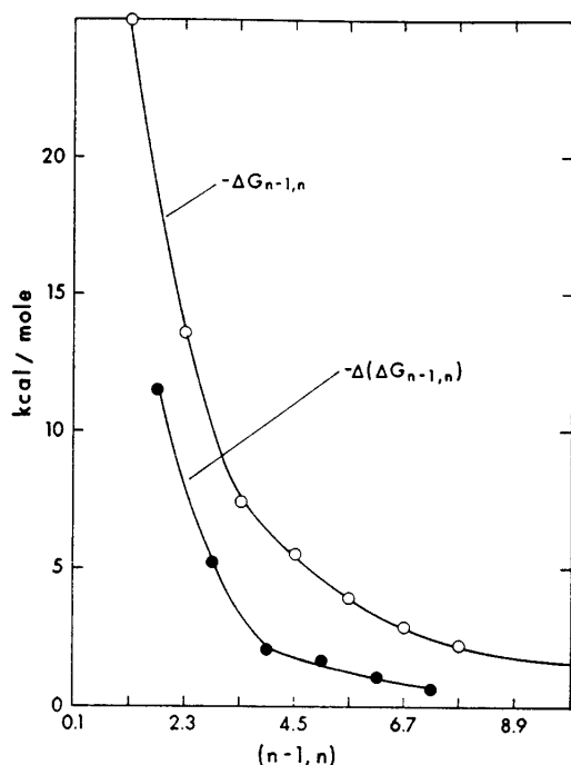
Figure 5. Plot of \Delta G^\circ_{n-1,n} and \Delta(\Delta G^\circ_{n-1,n}) at 300°K vs. n-1, n . Standard state of water vapor is 1 atm. Decrease of free-energy changes is quite regular showing that stabilities of clusters change quite regularly. A possible break is indicated between 3,4 and 4,5. This could be due either to crowding in the first "shell" or transition to an outer "shell."
