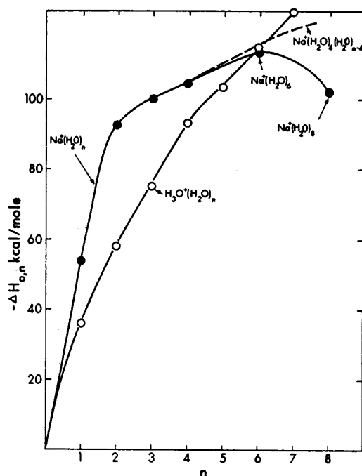
Figure 8. Plot of summed enthalpies of hydration \Delta H_{0,n} . The enthalpies for \text{Na}^+(\text{H}_2\text{O})_n and \text{Na}^+(\text{H}_2\text{O})_4(\text{H}_2\text{O})_{n-4} are based on calculations by Garrick. 18 The hydrogen ion data are from the present experiments. We have written \text{H}_3\text{O}^+(\text{H}_2\text{O})_n in order to facilitate comparison with sodium. The calculated sodium data illustrate that the buildup of a new shell need not show up as a discontinuity in \Delta H_{n-1,n} values since calculated \text{Na}^+(\text{H}_2\text{O})_6 and \text{Na}^+(\text{H}_2\text{O})_4 - (\text{H}_2\text{O})_2 have very similar enthalpies.
