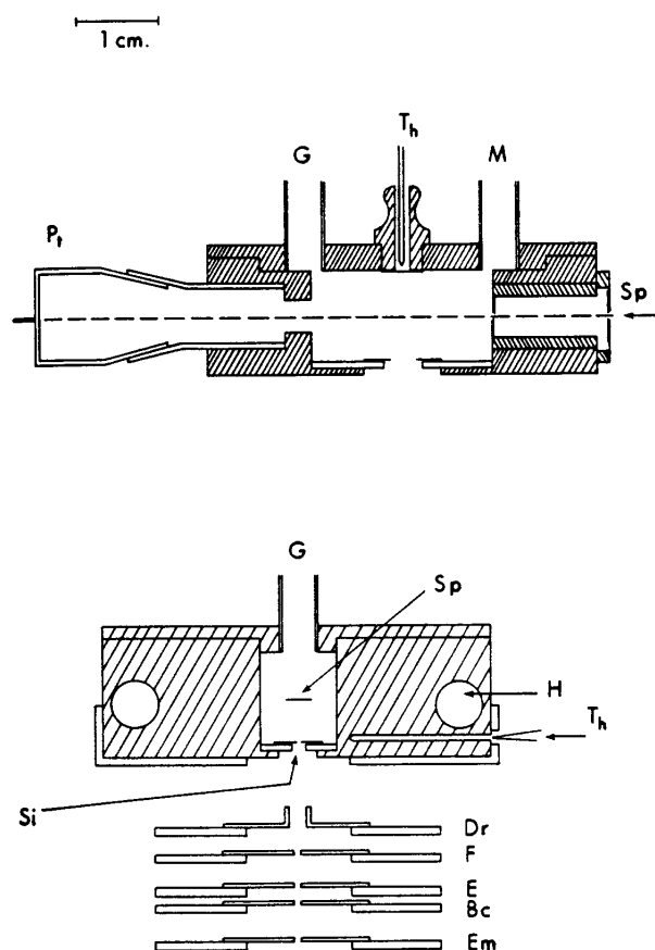
Figure 1. Front (upper) and side (lower) views of 100-keV proton beam ion source: G, gas inlet; Th, thermocouple; M, to manometer; P i , proton trap; Sp, proton entrance slit, 15 \mu wide; Si, ion exit slit, 5 \mu wide; H, heater. Electrodes: Dr, draw out; F, focus half-plates; E, beam-defining slit; Bc, beam center half-plates; Em, entrance slits into magnetic mass analyzer.
